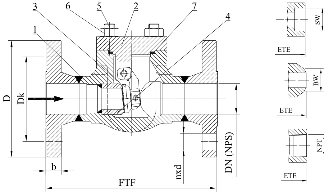
Drawing B.9.1 Parts and dimensions
