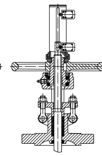
Limit switches
